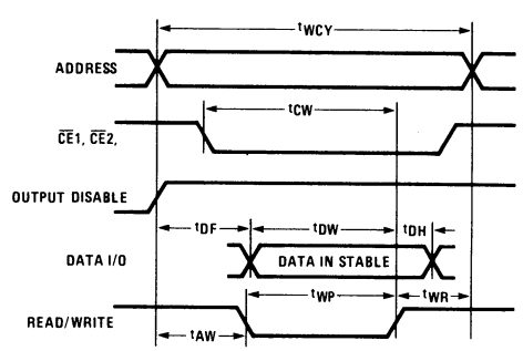
WRITE CYCLE
