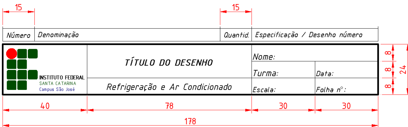
Figura 10.2: Legenda padr o do INSTITUTO FEDERAL – SANTA CATARINA – Campus S o Jos .
